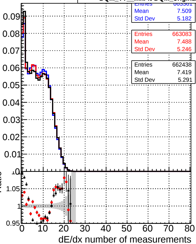
DQM_TT_mkFit-DQM_original_newwindows
