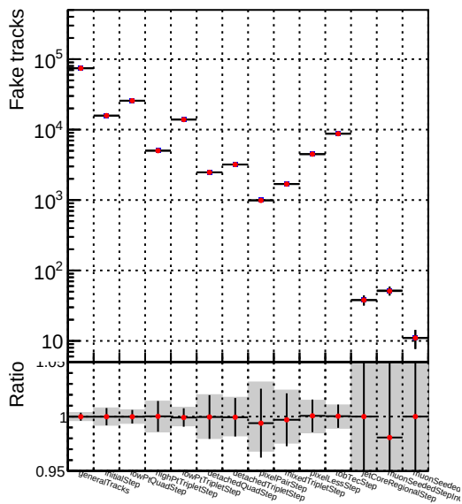
Number Label 1 DQM_V0001_R0000000001_Global_CMSSW_mkt50i3_RECO
