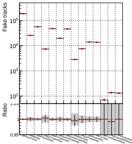
Number ● DQM_V0001 R0000000001 Global CMSSW_mkt50i3 RECO
