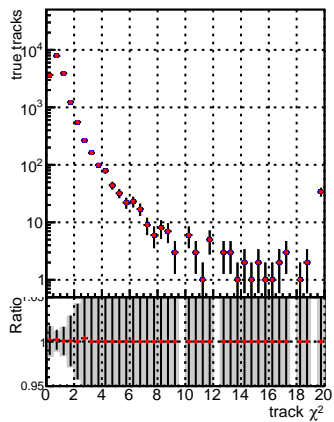
N of reco track vs. \chi^2 —●— DQM_V0001_R000000001_Global_CMSSW_mkt502_RECO —●— DQM_V0001_R000000001_Global_CMSSW_mkt503_RECO
