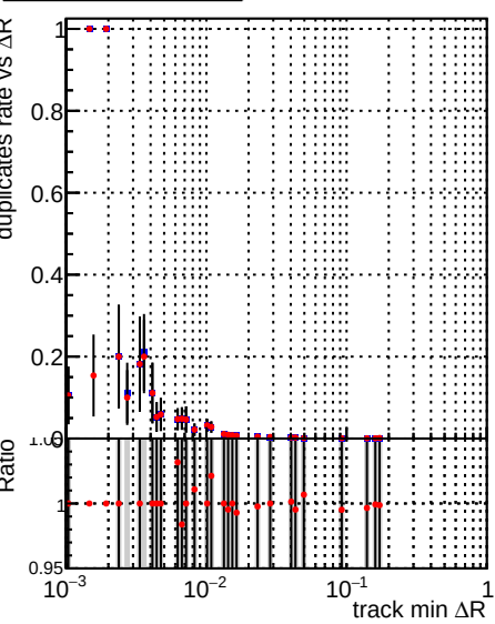
Legend: DQM_V0001_R000000001_Global_CMSSW_mkt502_RECO (blue line with error bars), DQM_V0001_R000000001_Global_CMSSW_mkt50i3_RECO (red line with error bars)
