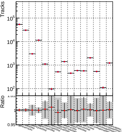
DQM_V0001_R000000001_Global_CMSSW_mkt502_RECO
