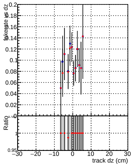
—●— DQM_V0001_R0000000001 Global CMSSW_mkt502_RECO —●— DQM_V0001_R0000000001 Global CMSSW_mkt50i3_RECO
