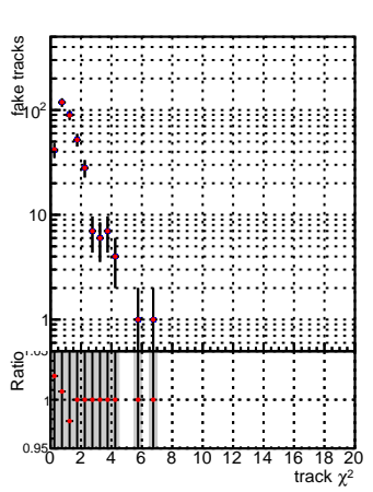
N of reco track vs. \chi^2 —●— Global_CMSSW_mkt502_RECO —●— Global_CMSSW_mkt503_RECO —○— DQM_V0001_R000000001 —○— DQM_V0001_R000000001
