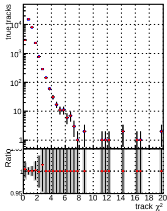
1__Global__CMSSW_mktt50i3_RECO
