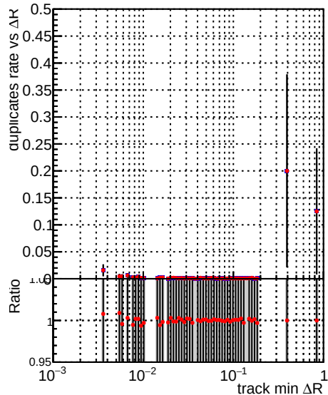
—●— DQM_V0001_R000000001_Global_CMSSW_mkt502_RECO —●— DQM_V0001_R000000001_Global_CMSSW_mkt50i3_RECO
