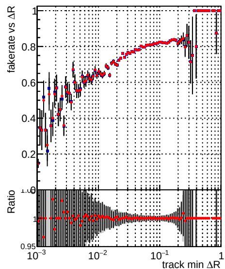
—●— DQM_V0001_R000000001_Global_CMSSW_mkt502_RECO —●— DQM_V0001_R000000001_Global_CMSSW_mkt50i3_RECO
