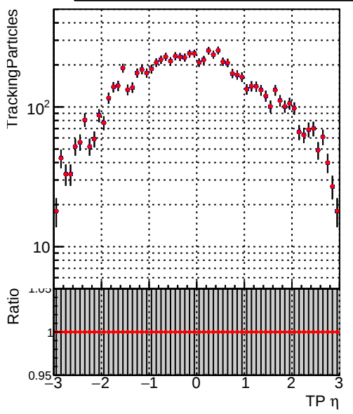
N of simulated tracks vs \eta Legend: DQM_V0001_R000000001_Global_CMSSW_mkt502_RECO (blue squares), DQM_V0001_R000000001_Global_CMSSW_mkt50i3_RECO (red diamonds)
