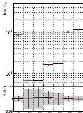
N of reco track vs. \chi^2 —●— DQM_V0001_R0000000001_Global_CMSSW_mkt502_RECO —●— DQM_V0001_R0000000001_Global_CMSSW_mkt503_RECO
