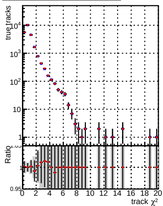
N of reco track vs. \chi^2 —●— DQM_V0001_R0000000001_Global_CMSSW_mkt502_RECO —●— DQM_V0001_R0000000001_Global_CMSSW_mkt503_RECO
