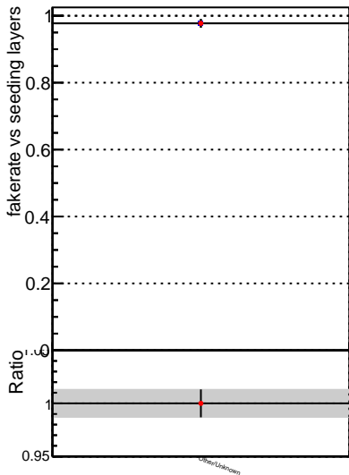
Fake rate vs. DQM_V0001_R000000001_Global_CMSSW_mkt502_RECO DQM_V0001_R000000001_Global_CMSSW_mkt50i3_RECO
