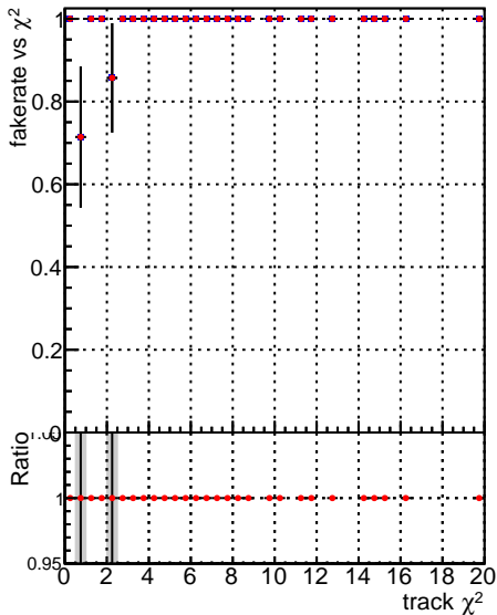
Fake rate vs. DQM_V0001_R000000001_Global_CMSSW_mkt502_RECO DQM_V0001_R000000001_Global_CMSSW_mkt50i3_RECO
