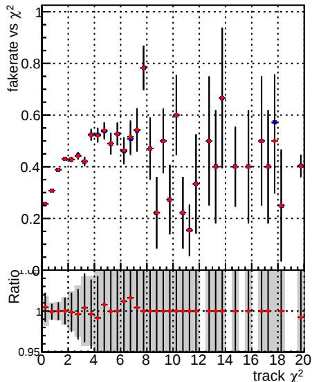
Fake rate vs. —•— DQM_V0001_R0000000001_Global_CMSSW_mkt502_RECO —•— DQM_V0001_R0000000001_Global_CMSSW_mkt503_RECO
