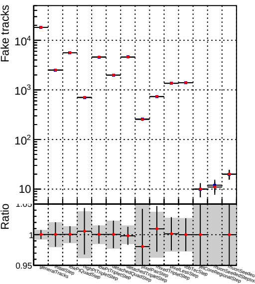
Number Label 1 DQM_V0001_R000000001_Global_CMSSW_mkt50i4_RECO
