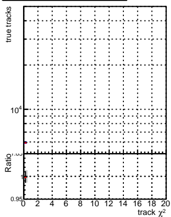
N of reco track vs. \chi^2 for DQM_V0001_R000000001_Global_CMSSW_mkt5017_RECO and DQM_V0001_R000000001_Global_CMSSW_mkt5014_RECO
