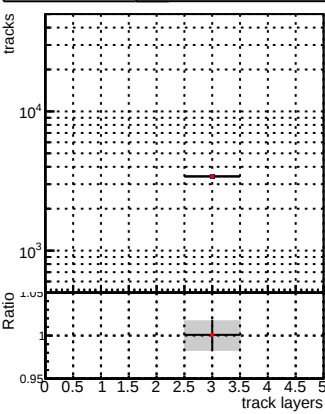
N of reco track vs l
