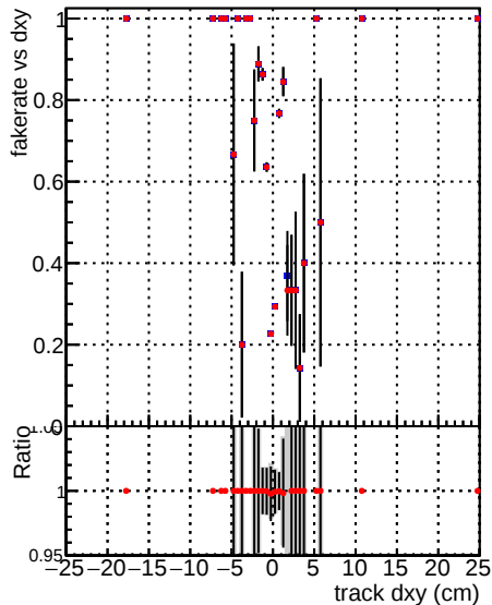
Fake rate vs d DQM_V0001_R0000000001 Global CMSSW_mkt50i7_RECO Global
