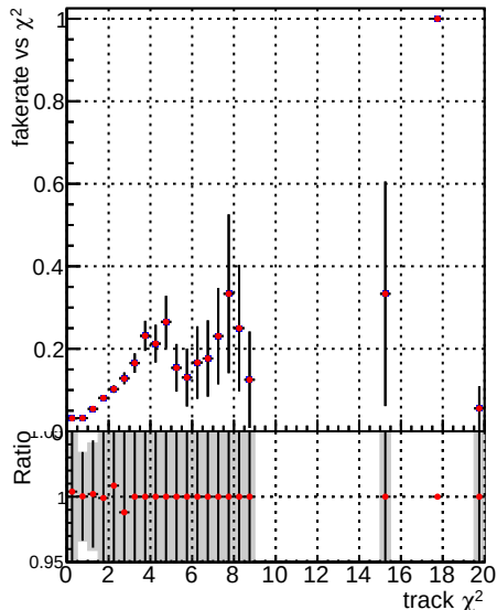
Fake rate vs. Legend Global CMSSW_mkt50i7 RECO Blue line with dots DQM_V0001_R0000000001 Global CMSSW_mkt50i7 Red line with dots DQM_V0001_R0000000001 Global CMSSW_mkt50i4
