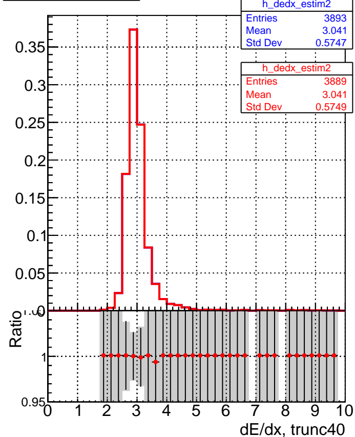
█ DQM_V0001_R000000001_Global_CMSSW_mkt50i7_RECO █ DQM_V0001_R000000001_Global_CMSSW_mkt50i4_RECO
