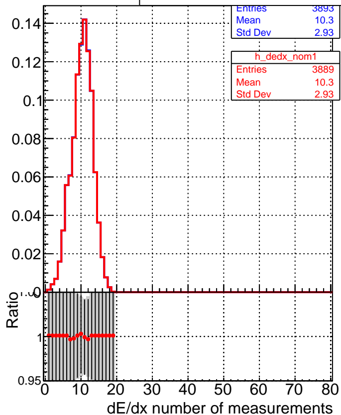
█ DQM_V0001_R000000001_Global_CMSSW_mkt50i7_RECO █ DQM_V0001_R000000001_Global_CMSSW_mkt50i4_RECO
