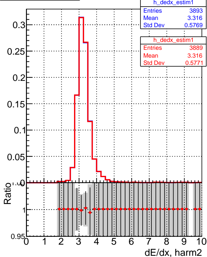
█ DQM_V0001_R000000001_Global_CMSSW_mkt50i7_RECO █ DQM_V0001_R000000001_Global_CMSSW_mkt50i4_RECO
