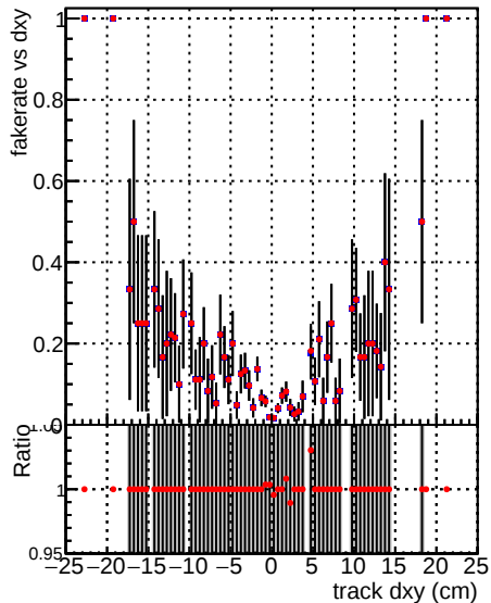
—●— DQM_V0001_R000000001 Global CMSSW_mkt50i7_RECO —●— DQM_V0001_R000000001 Global CMSSW_mkt50i4_RECO
