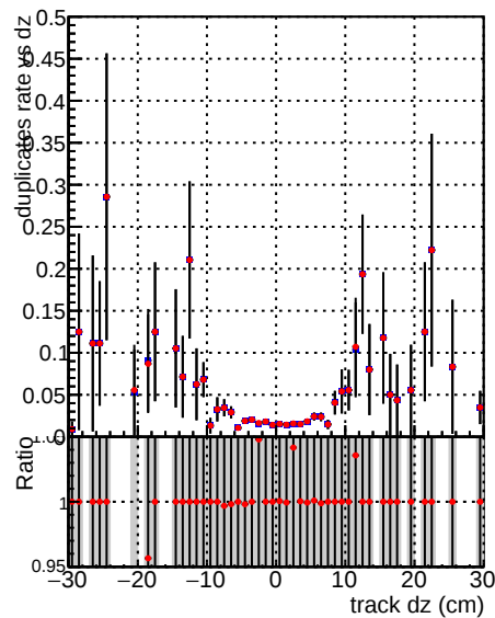
—●— DQM_V0001_R000000001 Global CMSSW_mkt50i7_RECO —●— DQM_V0001_R000000001 Global CMSSW_mkt50i4_RECO
