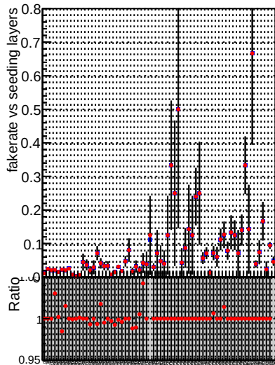
Fake rate vs. —●— DQM V0001_R000000001 Global CMSSW_mkt50i7 RECO —●— DQM V0001_R000000001 Global CMSSW_mkt50i4 RECO
