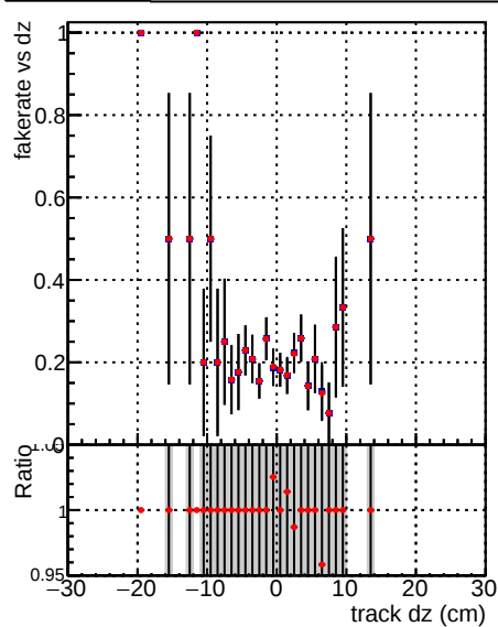
Fake rate vs dz —●— DQM_V0001_R0000000001_Global_CMSSW_mkt50i7_RECO —●— DQM_V0001_R0000000001_Global_CMSSW_mkt50i4_RECO
