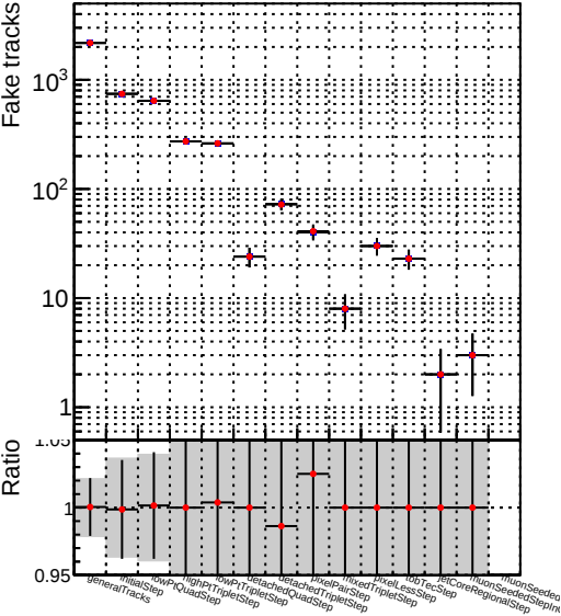
Number Label 1 DQM_V0001_R000000001_Global_CMSSW_mkt50i4_RECO
