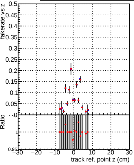
—•— DQM_V0001_R000000001_Global_CMSSW_mkt50i7_RECO —•— DQM_V0001_R000000001_Global_CMSSW_mkt50i4_RECO
