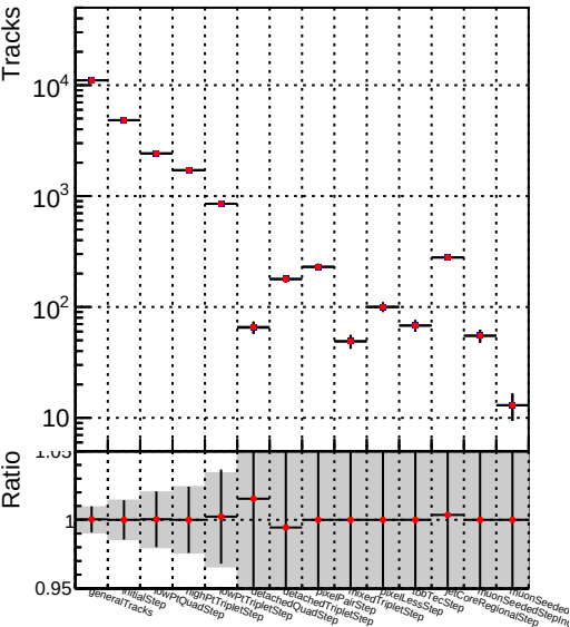
DQM_V0001_R000000001_Global_CMSSW_mkt50i7_RECO
