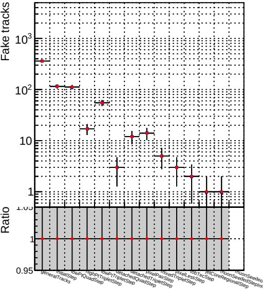
Numbe —● DQM_V0001_R000000001_Global_CMSSW_mkt50i4_RECO
