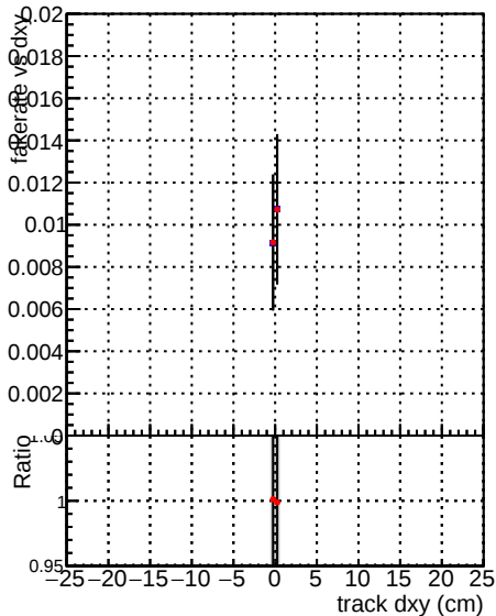
Global CMSSW_mkt50i7_RECO Fake rate vs d DQM_V0001_R0000000001 DQM_V0001_R0000000001 Duplicates Rate vs Dxy DQM_V0001_R0000000001 DQM_V0001_R0000000001 Pileup rate vs dxy DQM_V0001_R0000000001 DQM_V0001_R0000000001
