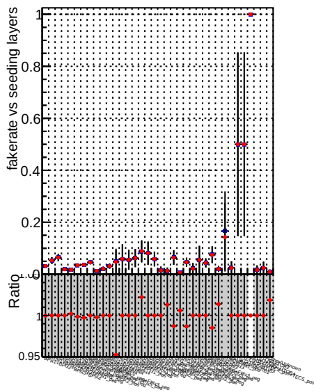
Fake rate vs. —•— DQM_V0001_R0000000001_Global_CMSSW_mkt50i7_RECO —•— DQM_V0001_R0000000001_Global_CMSSW_mkt50i4_RECO
