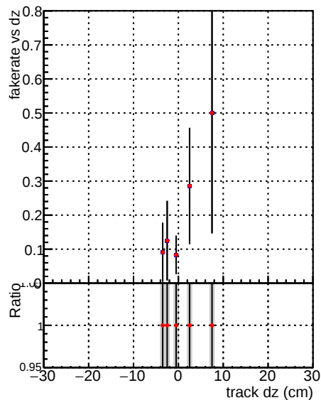
DQM_V0001_R0000000001 Global CMSSW_mkt50i7_RECO Fake rate vs d Blue dots Black line Red dots Duplicates Rate vs Dxy Blue dots Black line Red dots Pileup rate vs dxy Blue dots Black line Red dots
