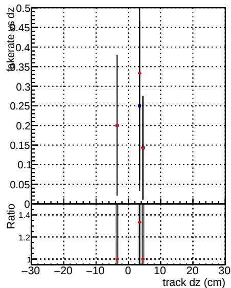
DQM V0001_R0000000001 Global CMSSW_mkt50i7_RECO Fake rate vs d Blue dots Blue dots Blue dots Fake rate vs dz Red dots Red dots Red dots
