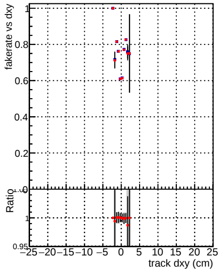
—●— DQM_V0001_R0000000001_Global_CMSSW_mkt50i7_RECO —●— DQM_V0001_R0000000001_Global_CMSSW_mkt50i4_RECO
