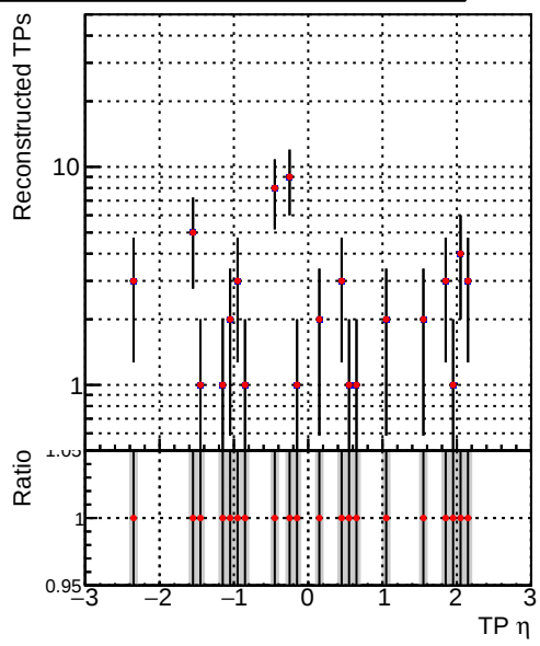
— DQM_V0001_R0000000001_Global_CMSSW_mkt50i7_RECO — DQM_V0001_R0000000001_Global_CMSSW_mkt50i4_RECO
