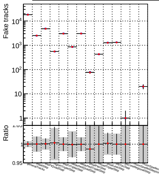
Number —●— DQM V0001 R0000000001 Global CMSSW mktt50i4 RECO
