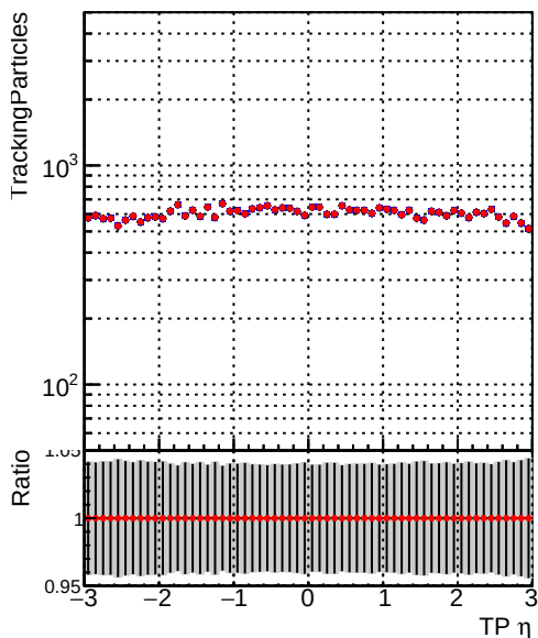
— DQM_V0001_R0000000001_Global_CMSSW_mkt50i7_RECO — DQM_V0001_R0000000001_Global_CMSSW_mkt50i4_RECO
