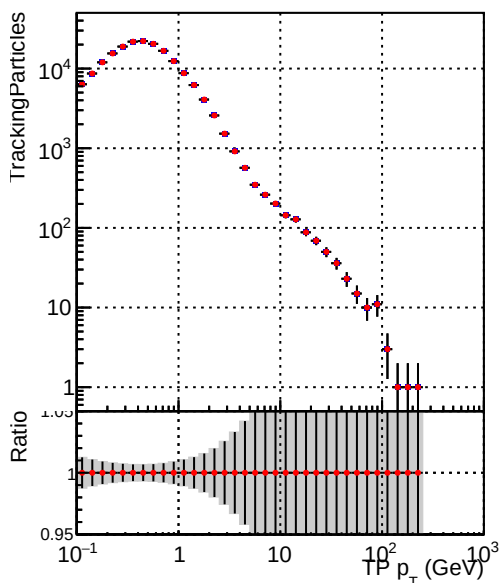
— DQM_V0001_R0000000001_Global_CMSSW_mkt50i7_RECO — DQM_V0001_R0000000001_Global_CMSSW_mkt50i4_RECO
