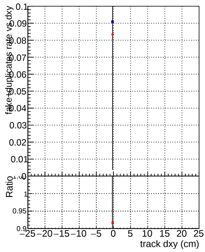
DQM_V0001_R000000001_Global_CMSSW_mkt50i7_RECO
