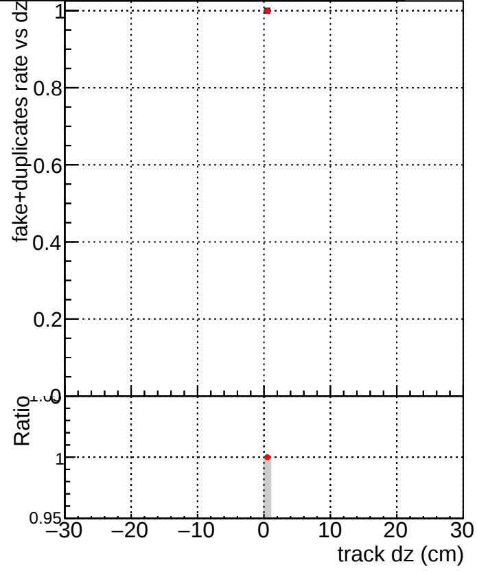
DQM_V0001_R000000001_Global_CMSSW_mkt50i7_RECO
