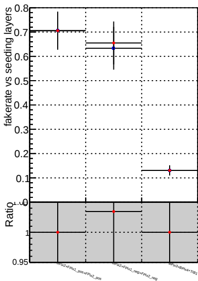
Fake rate vs. —•— DQM_V0001_R0000000001_Global_CMSSW_mkt50i7_RECO —•— DQM_V0001_R0000000001_Global_CMSSW_mkt50i4_RECO
