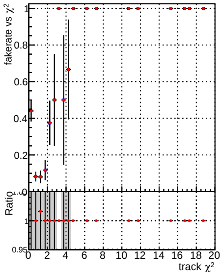
Fake rate vs. —•— DQM_V0001_R0000000001_Global_CMSSW_mkt50i7_RECO —•— DQM_V0001_R0000000001_Global_CMSSW_mkt50i4_RECO
