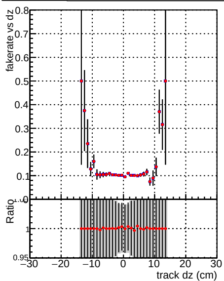
—●— DQM_V0001_R0000000001_Global_CMSSW_mkt50i7_RECO —●— DQM_V0001_R0000000001_Global_CMSSW_mkt50i4_RECO
