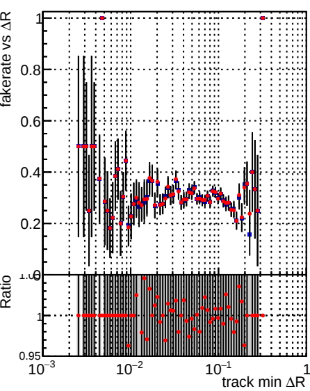
Legend: DQM_V0001_R000000001_Global_CMSSW_mkt50i7_RECO (blue line with error bars), DQM_V0001_R000000001_Global_CMSSW_mkt50i4_RECO (red line with error bars)
