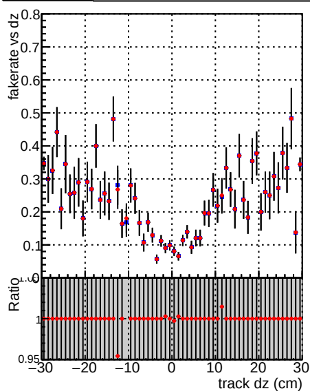
—●— DQM_V0001_R0000000001 Global CMSSW_mkt50i7_RECO —●— DQM_V0001_R0000000001 Global CMSSW_mkt50i4_RECO
