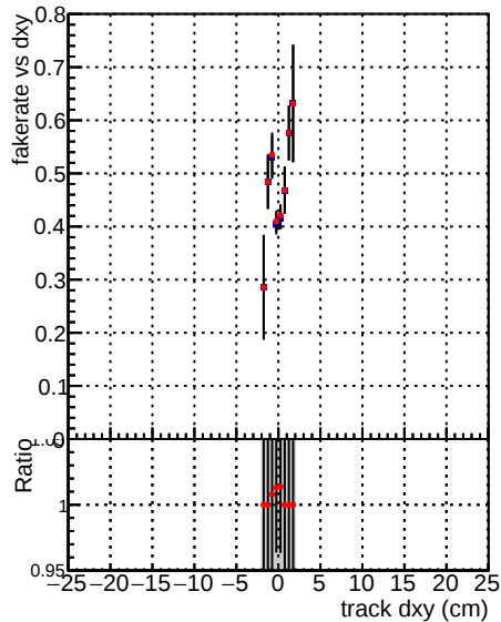
Legend Global CMSSW_mkt50i7_RECO Fake rate vs d Blue dots with error bars DQM_V0001_R0000000001 Global Red dots with error bars DQM_V0001_R0000000001 CMSSW_mkt50i4_RECO
