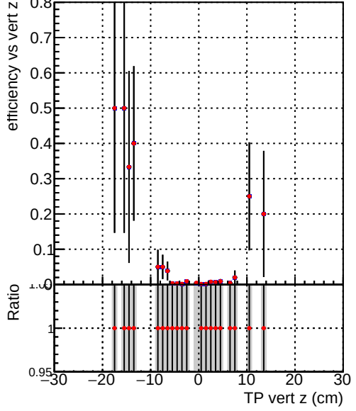
Efficiency vs. TP vert z (cm) for DQM_V0001_R000000001_Global_CMSSW_mkt50i7_RECO (blue) and DQM_V0001_R000000001_Global_CMSSW_mkt50i4_RECO (red).
