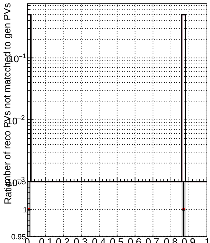
RecoPVAssoc2GenPVNotMatched_Purity
