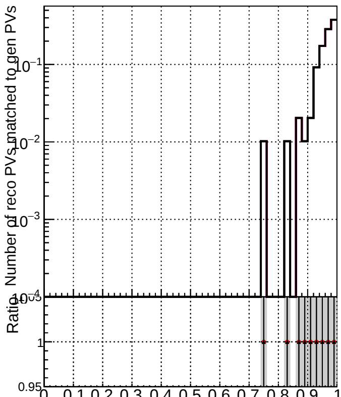
RecoPVAssoc2GenPVMatched_Purity
