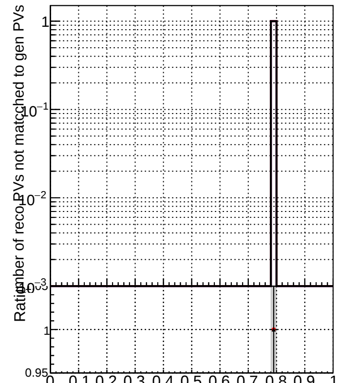
RecoPVAssoc2GenPVnotmatched_missing
