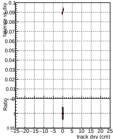
DOM_V0001 R0000000001 Global CMSSW_mkt5017 RECO Fake rate vs d Duplicates rate vs dz Pileup rate vs dz
