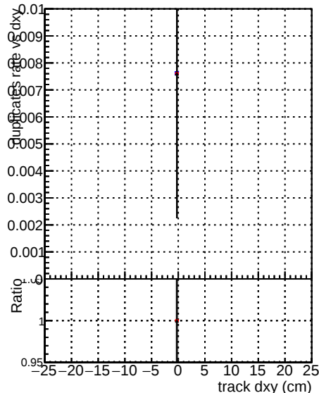
DOM V0001 DOM V0001 DOM V0001 Global Global CMSSW mkt5017 RECO CMSSW mkt5018 RECO Fake rate vs d 0.000000001 0.000000001 0.000000001 0.000000001 0.000000001 0.000000001 0.000000001 Duplicates Rate vs Dxy 0.000000001 0.000000001 0.000000001 0.000000001 0.000000001 0.000000001 0.000000001 Pileup rate vs dxy 0.000000001 0.000000001 0.000000001 0.000000001 0.000000001 0.000000001 0.000000001
