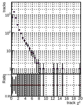
N of reco track vs. \chi^2 BQM V0001 R0000000001 Global CMSSW mkt5017 RECO BQM V0001 R0000000001 Global CMSSW mkt5018 RECO BQM V0001 R0000000001 Global CMSSW mkt5019 RECO
