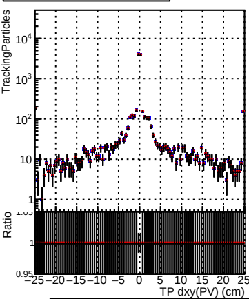
DQM_V0001_R000000001_Global_CMSSW_mkt50i4_RECO DQM_V0001_R000000001_Global_CMSSW_mkt50i5_RECO DQM_V0001_R000000001_Global_CMSSW_mkt50i6_RECO
