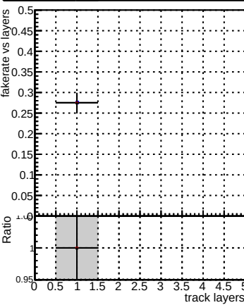
Fake rate vs layers
