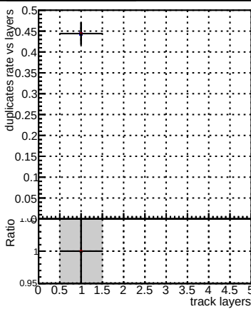
Duplicates Rate vs layers
