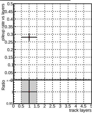
Pileup rate vs layers
