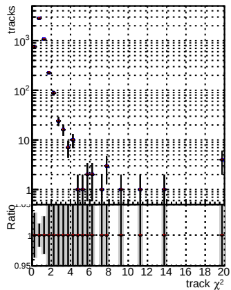
N of reco track vs. BQM V0001 R0000000001 Global CMSSW mkt5014 RECO BQM V0001 R0000000001 Global CMSSW mkt5015 RECO BQM V0001 R0000000001 Global CMSSW mkt5016 RECO
