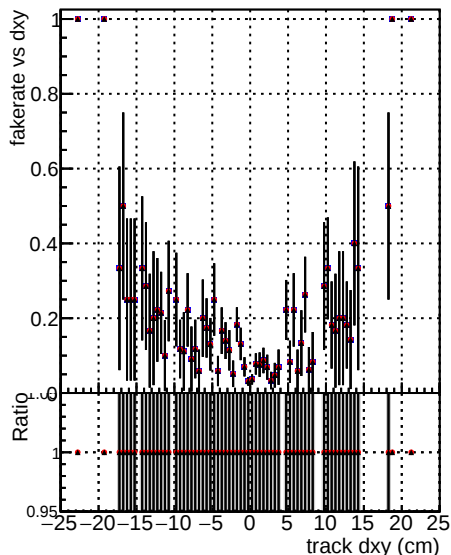
DOM V0001 DOM V0001 Global CMSSW mkt5014 RECO CMSSW mkt5016 RECO Fake rate vs d DOM V0001 DOM V0001 Global CMSSW mkt5014 RECO CMSSW mkt5016 RECO
