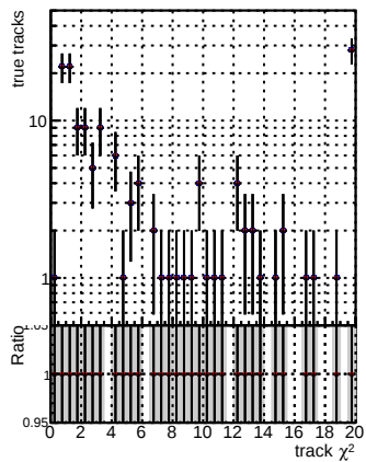
Ns of associated (recoToSim) tracks vs normalized \chi^2
